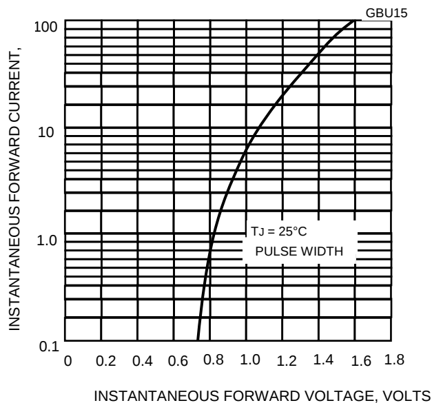
FIG.4-TYPICAL FORWARD CHARACTERISTICS
